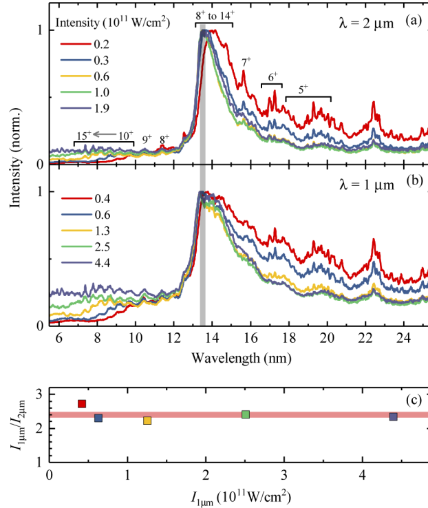
Fig. 3. Spectra from plasma produced from a planar solid tin target irradiated with laser pulses at various intensities of the (a) 2-μm driver (4.8 ns pulse duration, Gaussian spot size of 72×128 μm). The emission features attributed to the various Sn ions are labeled by the respective charge state. (b) Spectra from tin plasma driven by a 1-μm-beam (4.4 ns pulse duration, Gaussian spot size of 66×66 μm). The gray vertical band indicates a 2% bandwidth centered at 13.5 nm. (c) Ratio of intensities of 1- and 2-μm drive laser beams needed to obtain spectra with matching short-wavelength features. The red line indicates the average ratio.
