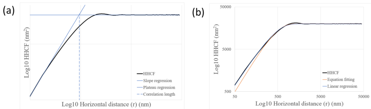
Figure 7 - (a) Linear regressions for HHCF and (b) HHCF fitting functions for SIMU
