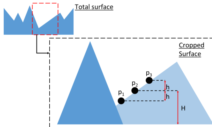
Figure 13 - Downward, the cropped surface from “Total surface”, upward. H and h are respectively the off-set height and the distance between two following points.
