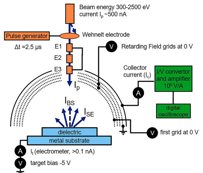
Fig. 2. Schematic overview of the collector-only SEY measurement setup.
