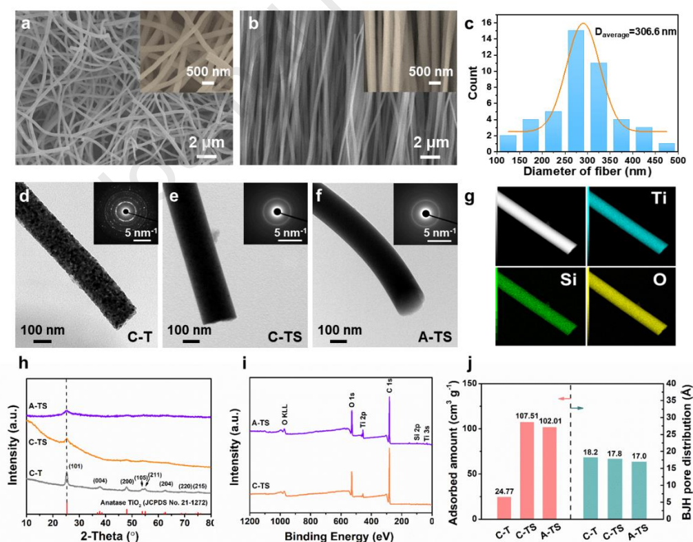
Fig. 2. Morphological and structural characterizations of various samples. Field emission scanning electron microscopy (FE-SEM) images of (a) C-TS and (b) A-TS membranes; (c) the diameter
