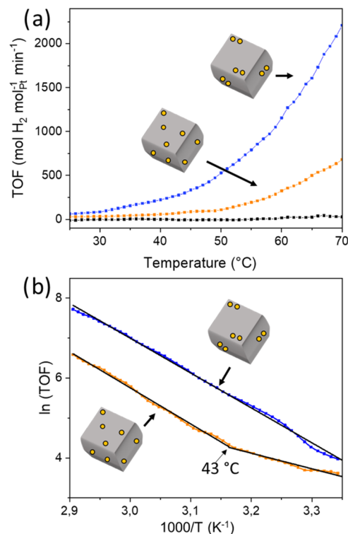
Figure 3. (a) Ammonia borane hydrolysis experiments at different temperatures for the support (black), the SAC (orange), and the DAC (blue). (b) Arrhenius plot of figure (a); the support was left out for clarity. These are high-precision measurements: Each point on the curve represents a window average of 25 data points, and each curve is an average of duplicate experiments.
