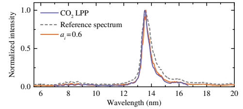
FIG. 5. Comparison of the transported reference spectrum using Eq. (3) with a_i = 0.6 , and the spectral emission from a \text{CO}_2 -laser-driven plasma.
