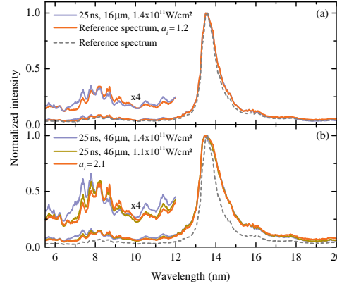
FIG. 3. Comparison of the reference spectrum and radiation transported reference spectrum with the measured spectra. The reference spectrum was transported using Eq. (3) together with the relative optical depth as determined in Fig. 2. (a) Increasing laser pulse duration (b) Increasing laser pulse duration and droplet size. An additional spectrum is shown measured at lower laser intensity of 1.1 \times 10^{11} \text{ W/cm}^2 providing a better match with the radiation transported spectrum in the 5 to 12 nm range.
