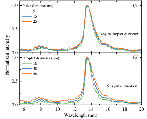
FIG. 1. Selection of emission spectra of Nd:YAG-laser-produced plasma from tin microdroplets irradiated at constant laser intensity of I = 1.4 \times 10^{11} \text{ W/cm}^2 while varying either (a) laser pulse duration or (b) droplet diameter.
