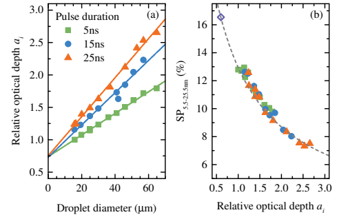
FIG. 4. (a) Dependency of the relative optical depth a_i on droplet diameter for various laser pulse durations as obtained, e.g., in Fig. 2. The solid lines show a linear extrapolation of the data toward zero droplet size. (b) Experimental values for spectral purity ( \text{SP}_{5.5-25.5\text{nm}} ) versus relative optical depth. The dashed line represents \text{SP}_{5.5-25.5\text{nm}} as calculated from the radiation transported reference spectrum. The open diamond symbol indicates the \text{SP}_{5.5-25.5\text{nm}} value of the radiation transported reference spectrum for a relative optical depth parameter a_i = 0.6 , a value obtained from comparison of the radiation transported reference spectrum with the emission of the \text{CO}_2 -laser-driven plasma as shown in Fig. 5 (see text).
